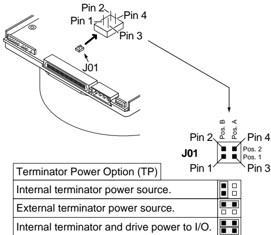
Figure 13. Setting terminator power jumpers on W models
