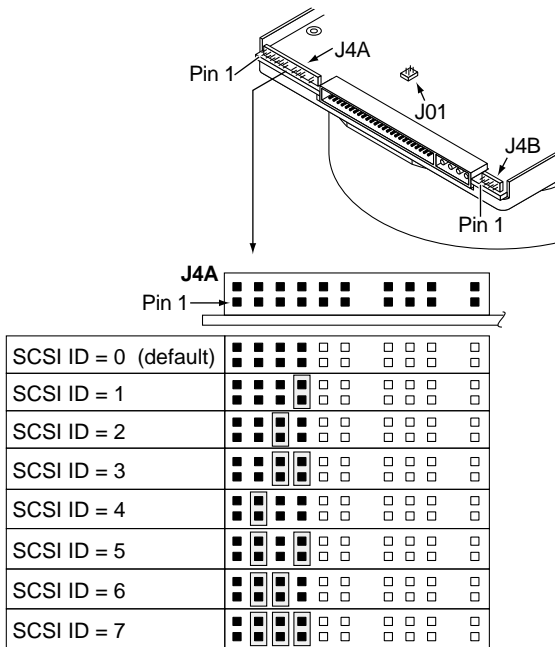
Figure 7. Setting the SCSI ID on N models
