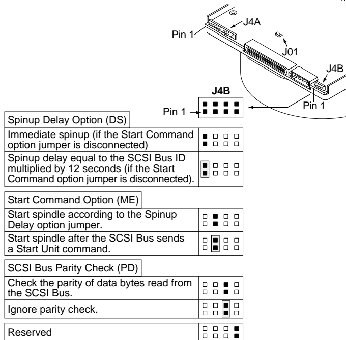
Figure 14. Additional jumper options
