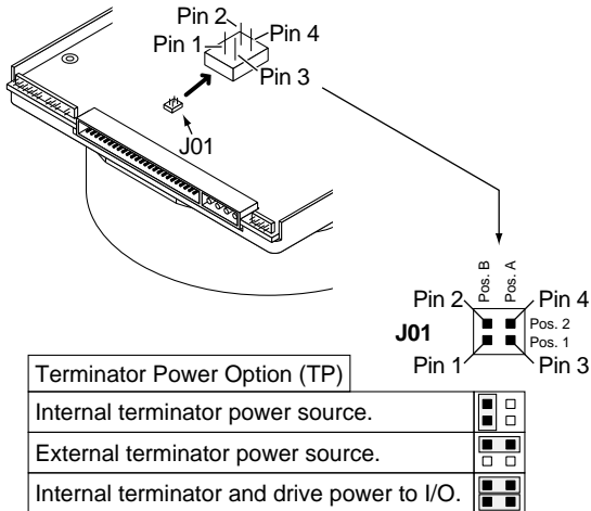
Figure 9. Setting terminator power jumpers on N models
