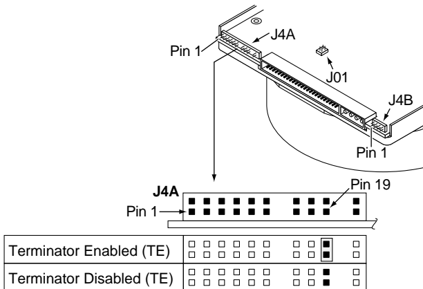
Figure 8. Terminating the drive
